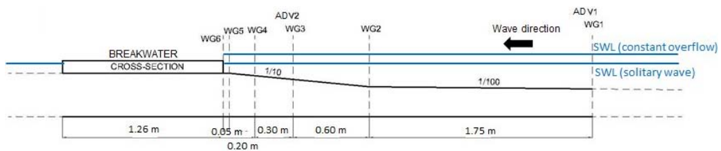
(a) Wave flume at PARI
