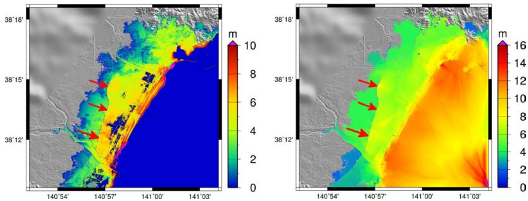
Fig. 10. The maximum flow depth (left panel) and the maximum surface elevation in the sea as well as the maximum inundation height on land (right panel) in Sendai area. Red arrows show the location of a road that reduces the tsunami inundation.
