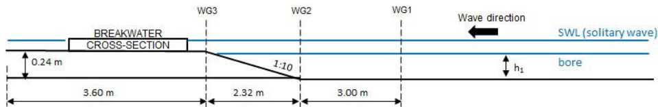
(b) Wave flume at TU-BS
